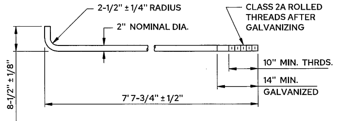
ANCHOR ROD DETAIL (SPEC. 3385 TYPE C)
