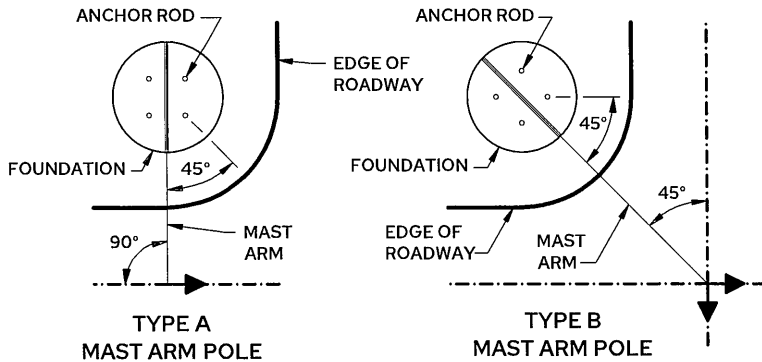
ANCHOR ROD PLACEMENT (WHEN USED WITH MAST ARM POLE)
