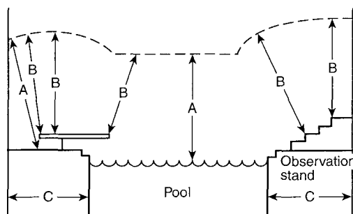
Figure 680.8 Clearances from pool structures.
