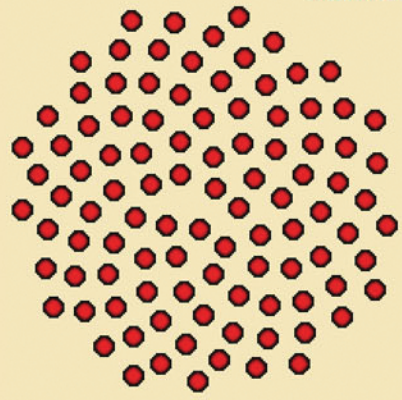
SUNFLOWER MODEL
