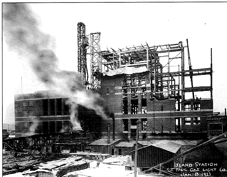
Figure 15. Island Station construction, looking east, January 8, 1923.
