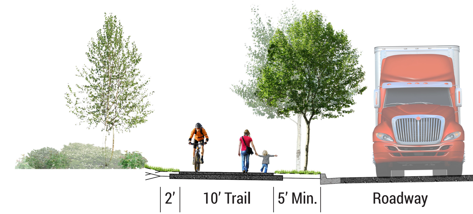
Barge Channel Road - Typ. Section B3
