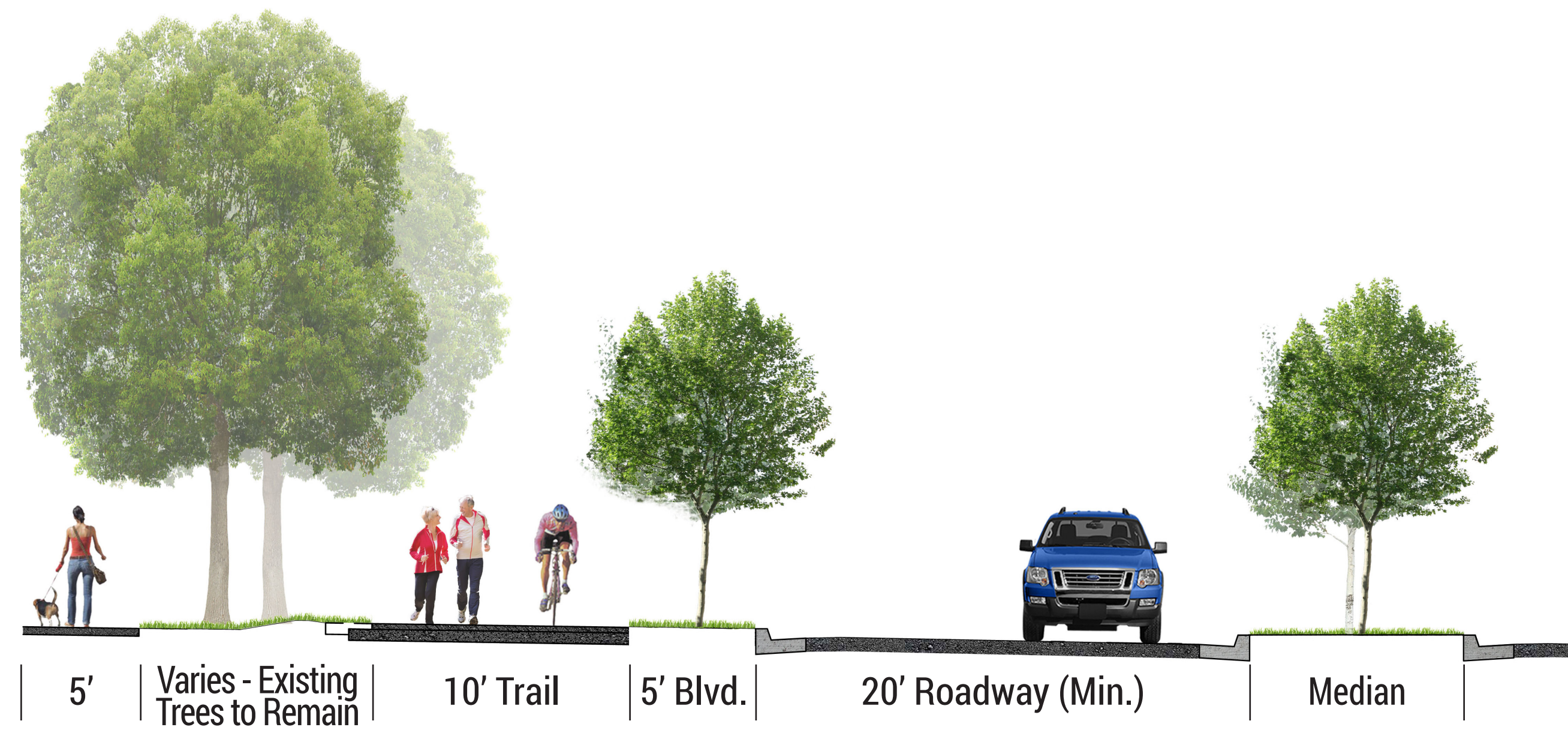
Plato Boulevard - Typ. Section P1
