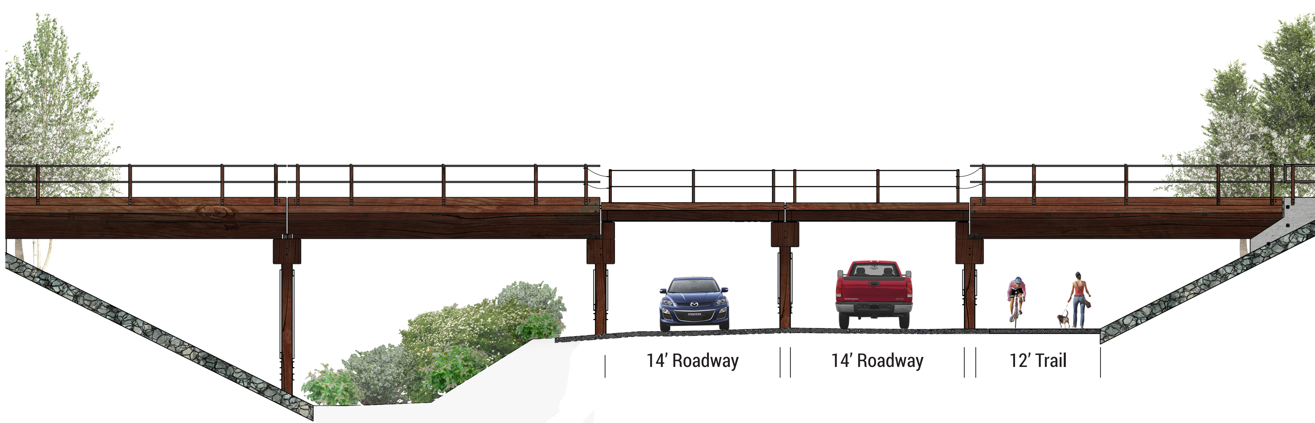
Lilydale - R&R Bridge Section
